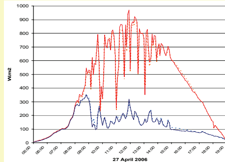
SPN1 Direct and Diffuse Outputs (solid traces) compared with a pair of Kipp CM6B pyranometers with solar tracking and shading disk (broken traces).
